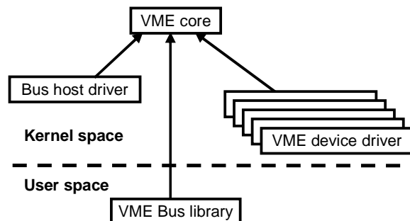
Figure 2: VME software layout for Linux 2.6
