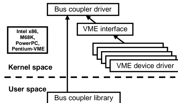
Figure 1: VME software layout for Linux 2.4
